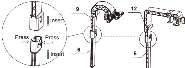
SEQUOIA SPIRIT® POOL SET
